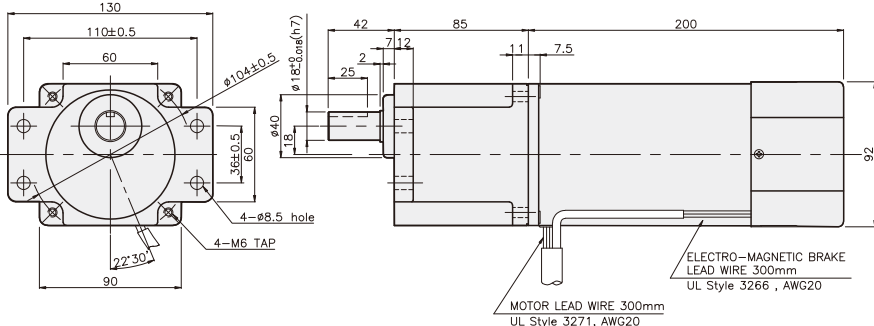
K9RP180F□-B + K9P□BUF
