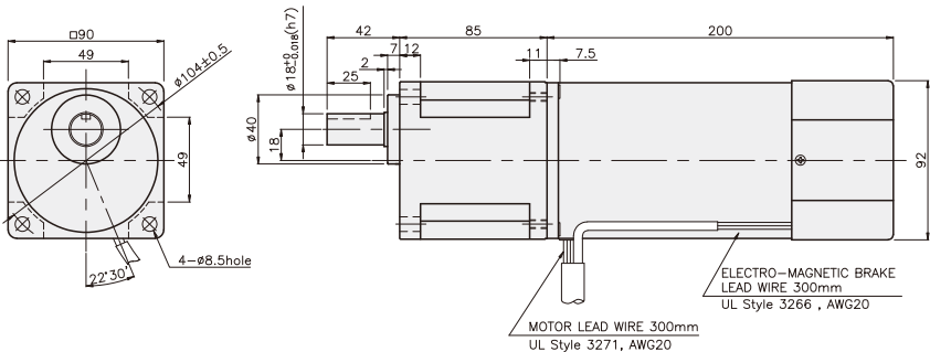
K9RP180F□-B + K9P□BU
